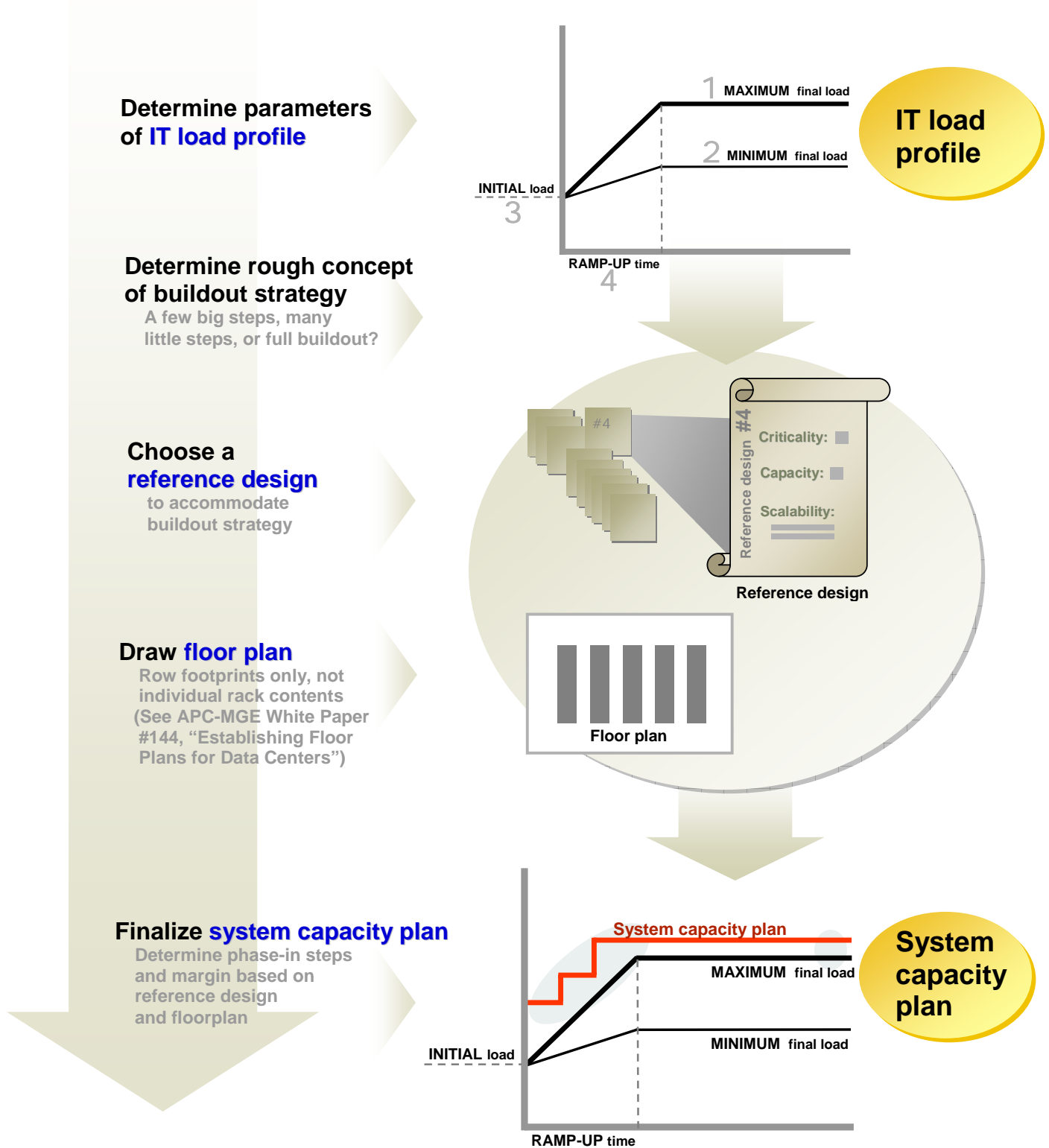
Figure 17 – Transformation of IT load profile into system capacity plan
