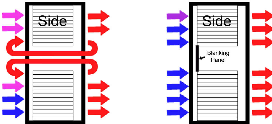
1A: without airflow management blanking panels
