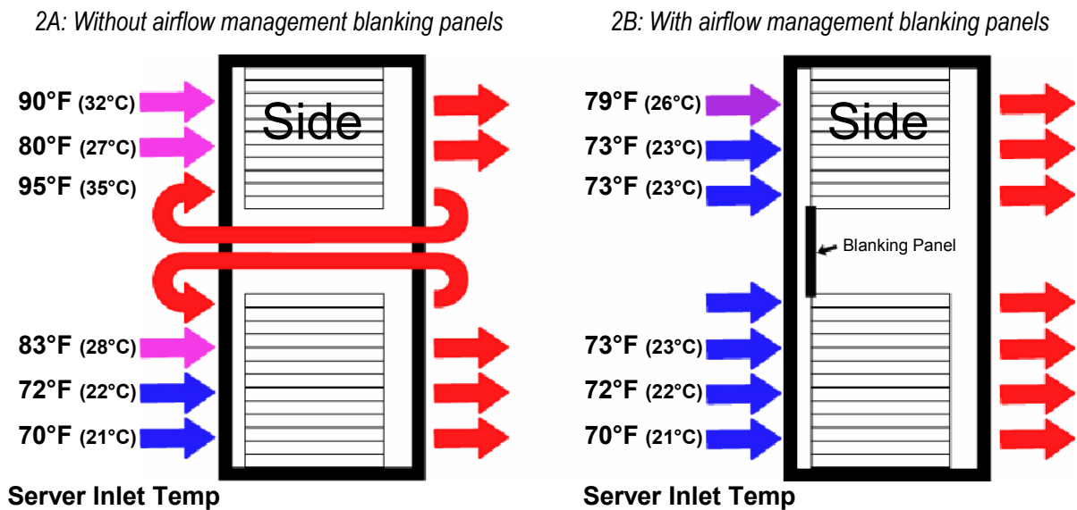
Figure 3 – Effect of installation of airflow management panel on server air inlet temperature
