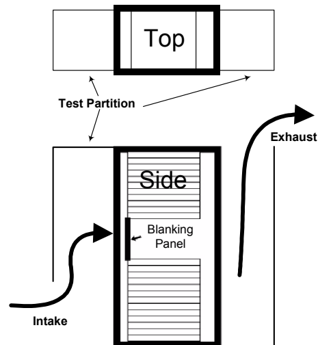
Figure A1 – Experimental setup
