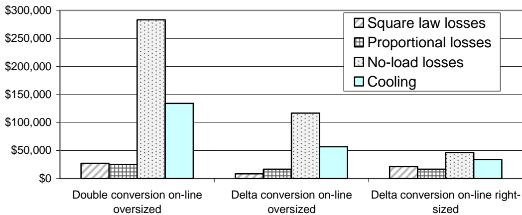
Figure 9 – 10 year cost breakdown of losses in a 1N architecture
