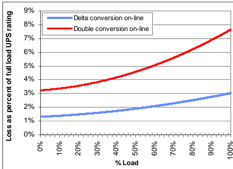
Figure A1 – Power loss curves for Delta conversion UPS and Double conversion UPS
