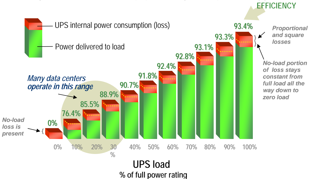
Figure 2 – Breakdown of total UPS input power showing where the power ultimately goes
