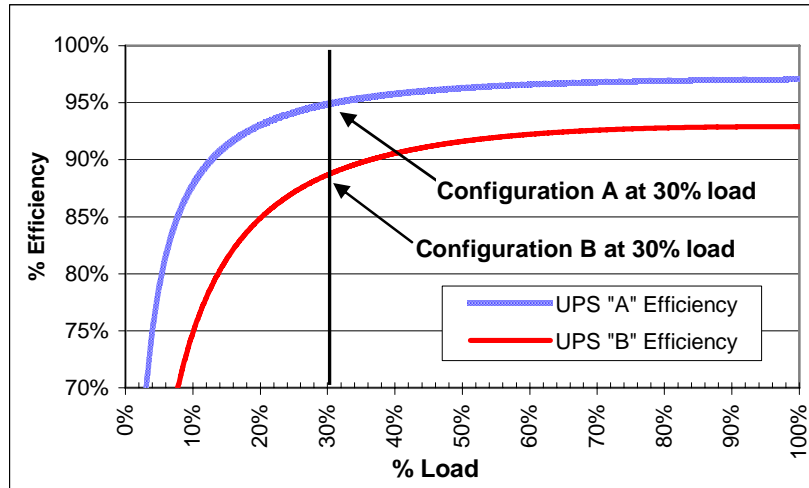
Figure 6 – Efficiency curves for delta conversion UPS “A” and double conversion UPS “B”
