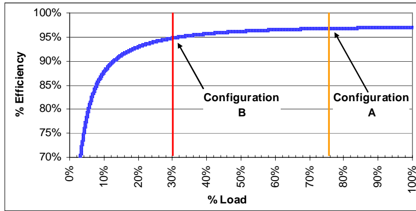
Figure 8 – Efficiency curve for 1MW delta conversion UPS
