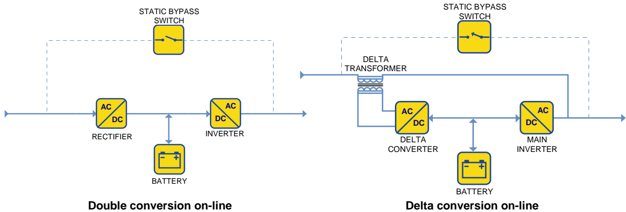
Figure 5 – Two “on-line” UPS power conversion technologies
