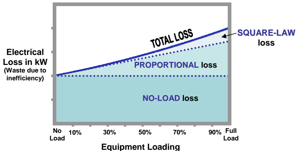
Figure 3 – Power loss graph
