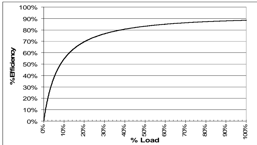
Figure 1 – UPS efficiency curve
