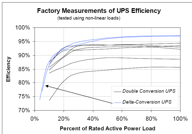
Figure 4 – Excerpt from EPRI UPS report (pg. 20)
