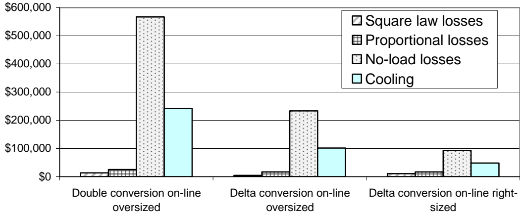
Figure 10 – 10 year cost breakdown of losses in a 2N architecture
