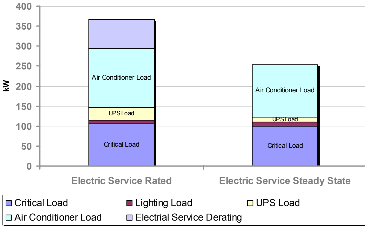
Figure 2 – Rated vs. steady-state electrical service power for a typical 100kW critical load. Electrical service rating is almost 4X the steady state critical load value
