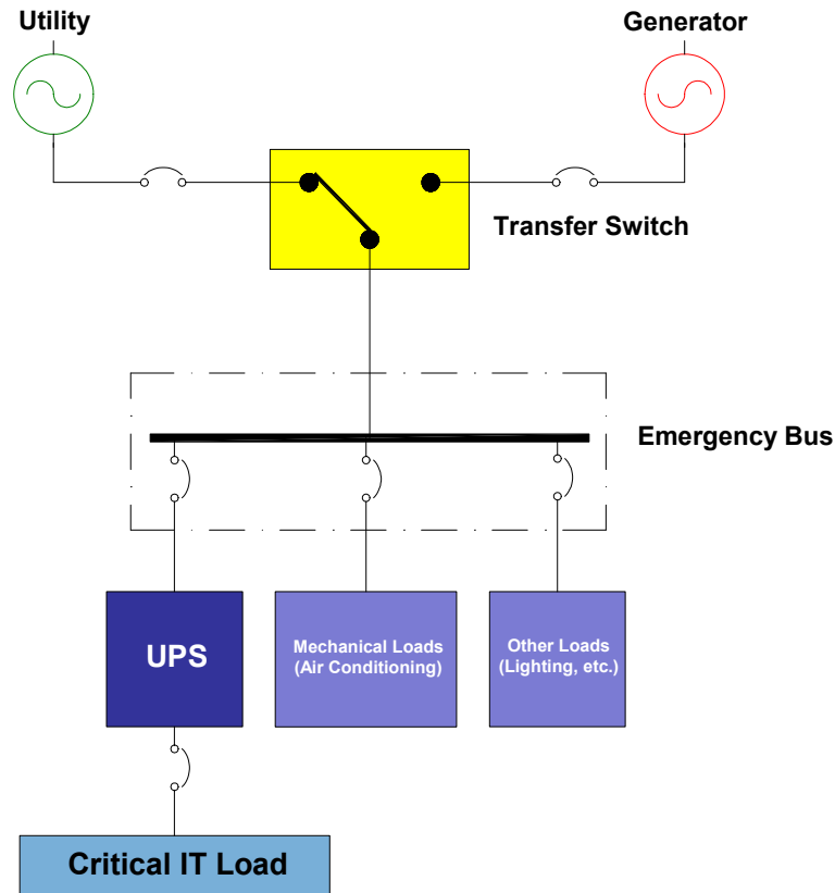
Figure 3 – Typical generator system
