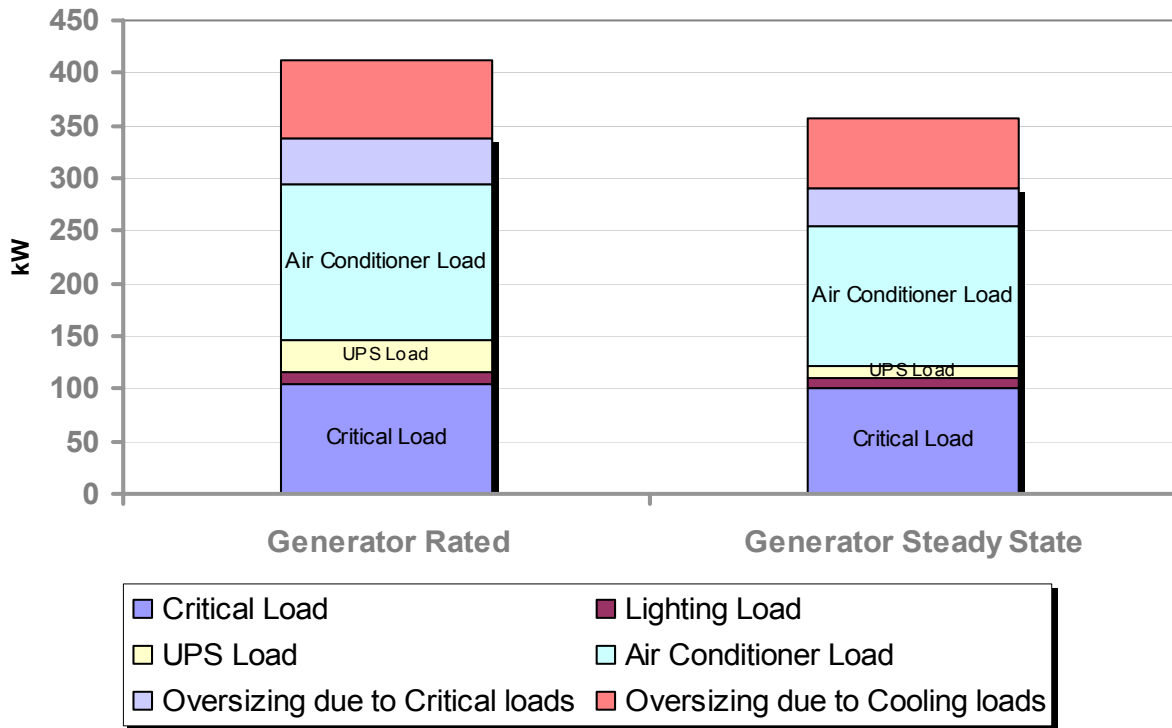
Figure 4 – Rated vs. Steady-State electrical generator power for a typical 100KW critical load. Electrical service rating is over 4X the steady state critical load value
