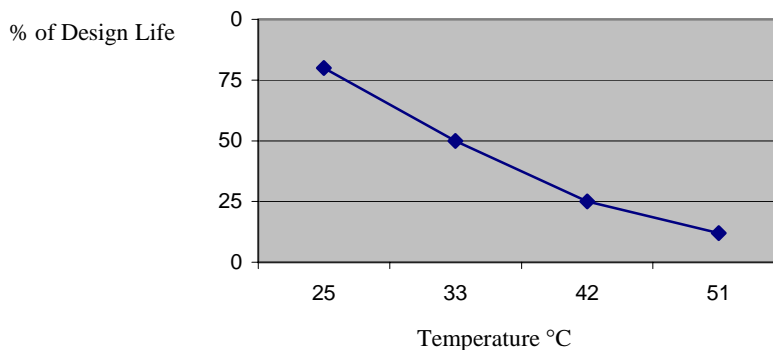
Figure 1 -- Operating temperature vs. battery life
