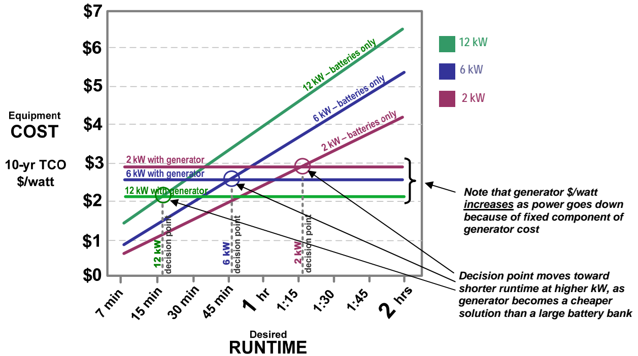
Figure 5 – Representative TCO analysis for three different UPS loads
