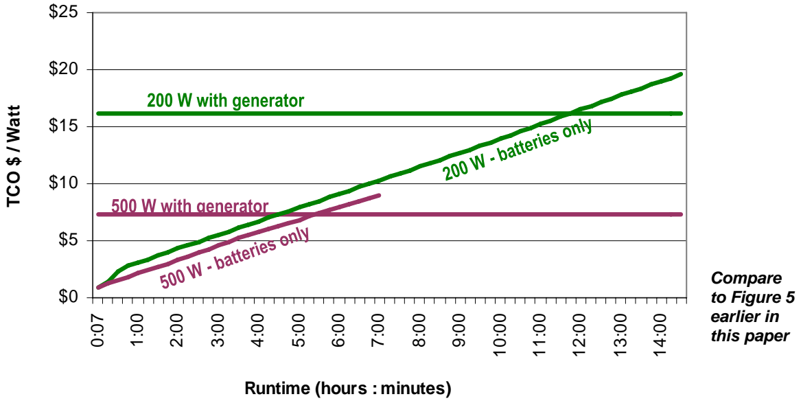
Figure A2 – UPS with batteries vs. UPS with generator – Based on actual pricing data for 200 W and 500 W loads
