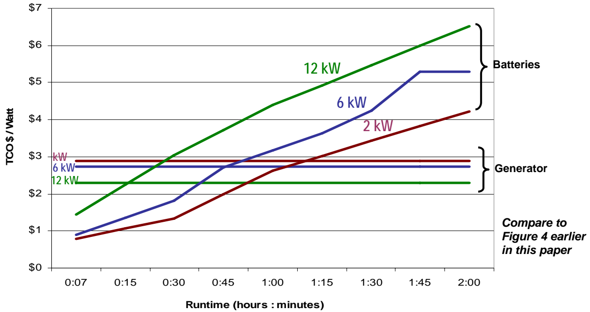
Figure A1 – UPS with batteries vs. UPS with generator – Based on actual pricing data for 2 kW, 6 kW and 12 kW loads
