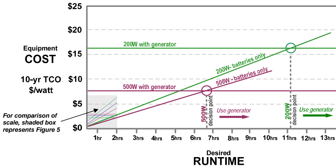
Figure 6 – At very low power, generator is not economical except for very long runtimes
