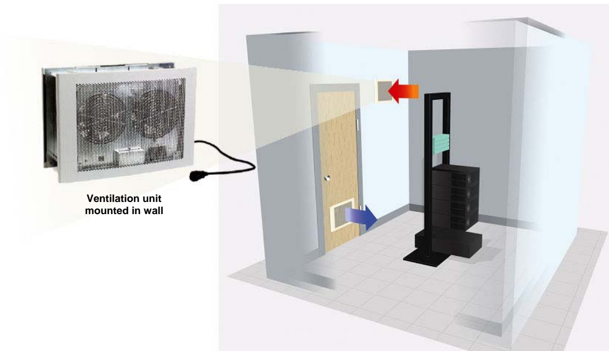
Figure 3 – Application of a wiring closet ventilation unit
